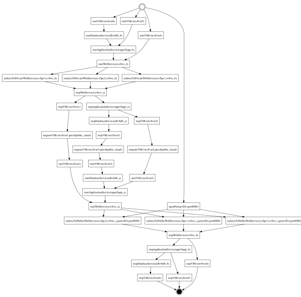
Figure 9: The generated workflow for cloud-burst problem.
